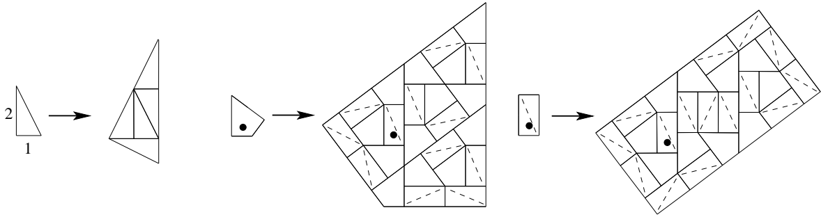
FIGURE 4. The substitution for the pinwheel tiling (left) and for the kite domino tiling (right). The dashed lines indicate how the dominos have to be dissected to obtain a pinwheel tiling. They are also needed to turn the global substitution rule for KD into a local one for its hull.
